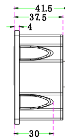
侧视图 Side view
